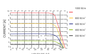
TYPICAL I-V CURVES
