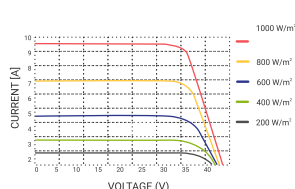
TYPICAL I-V CURVES
